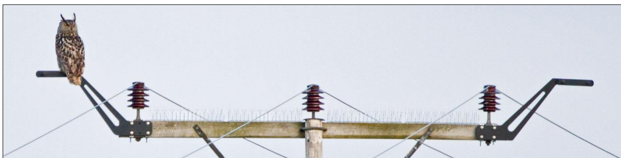
Eagle owl using specially developed perch, designed by scientists to help prevent electrocution of this species. © Karl-Otto Jacobsen
